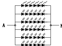
Backlight LED Circuit I_f=120\text{mA} ; V_f=19.6\text{V}
